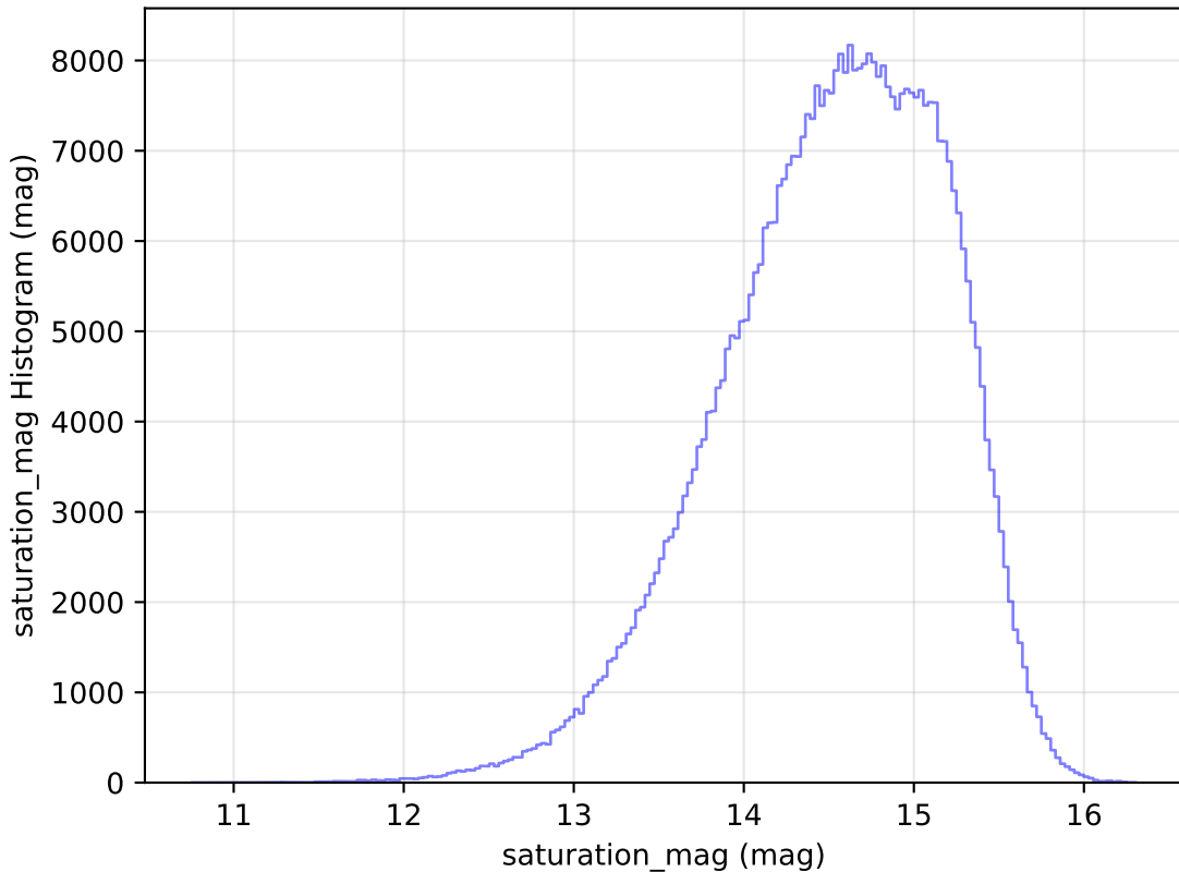
too_elab_r64_d3_giz_v3.4_10yrs WFD r band: saturation_mag Histogram
