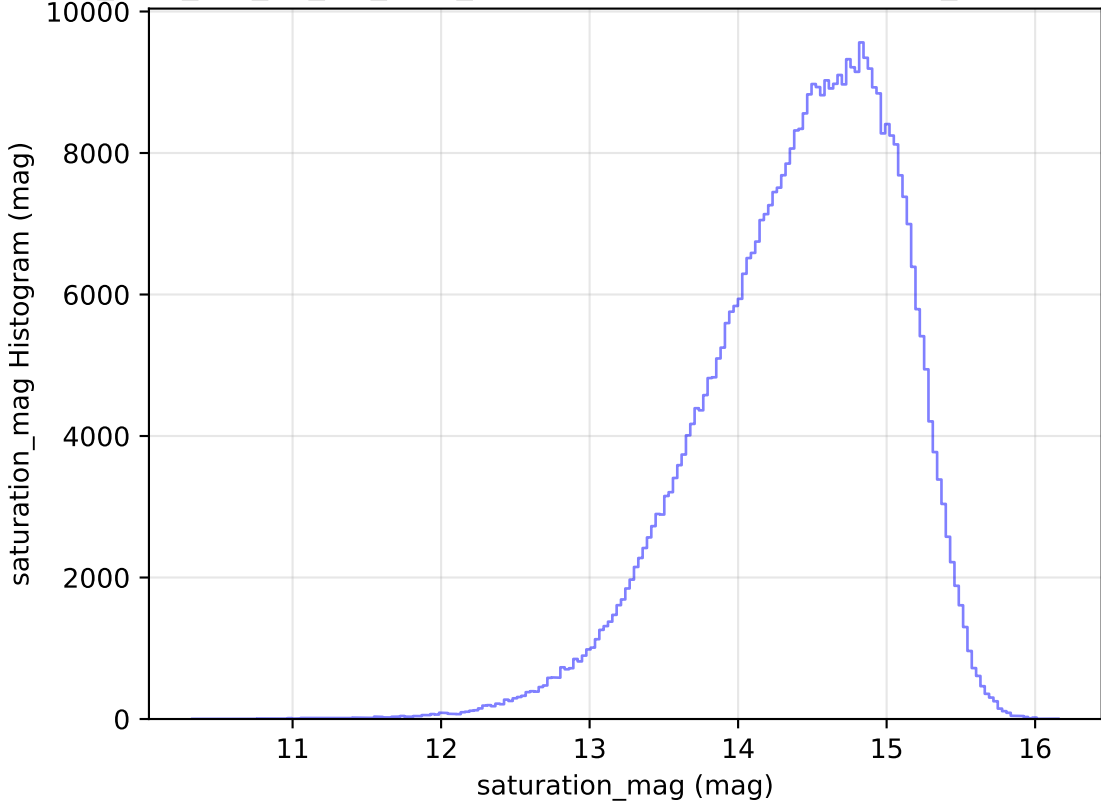
too_elab_r64_d3_giz_v3.4_10yrs WFD i band: saturation_mag Histogram
