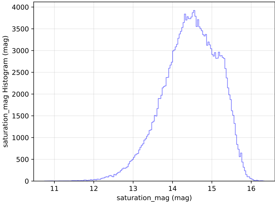
too_elab_r64_d3_giz_v3.4_10yrs WFD g band: saturation_mag Histogram
