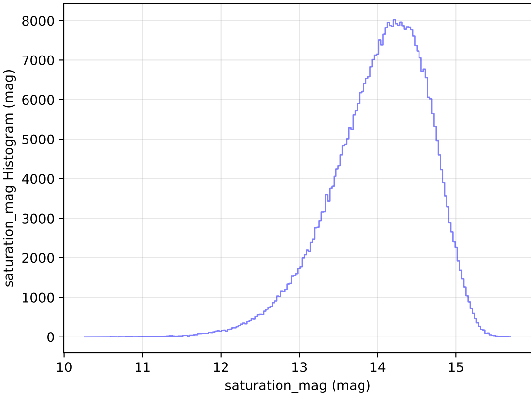
too_elab_r64_d3_giz_v3.4_10yrs All sky z band: saturation_mag Histogram
