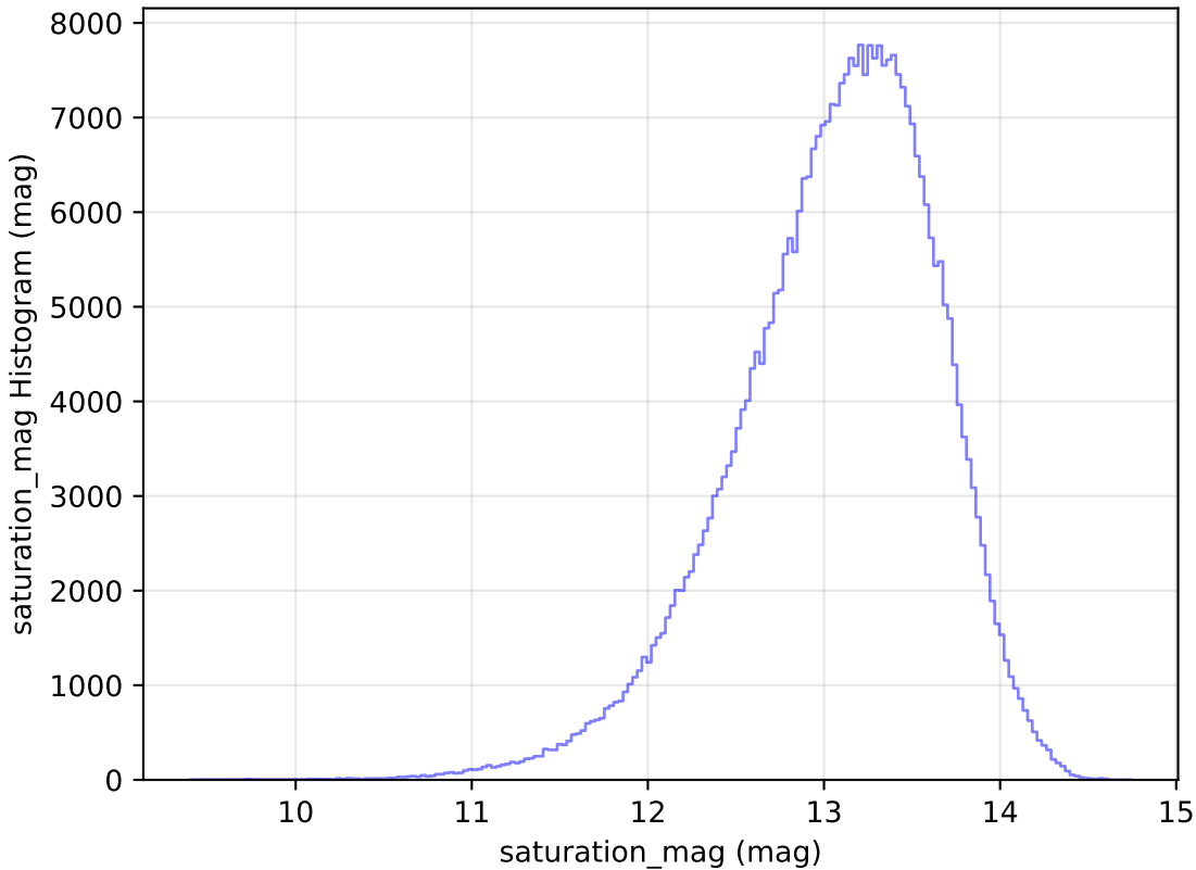
too_elab_r64_d3_giz_v3.4_10yrs All sky y band: saturation_mag Histogram
