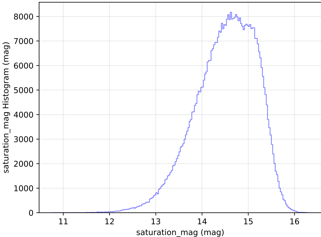
too_elab_r64_d3_giz_v3.4_10yrs All sky r band: saturation_mag Histogram
