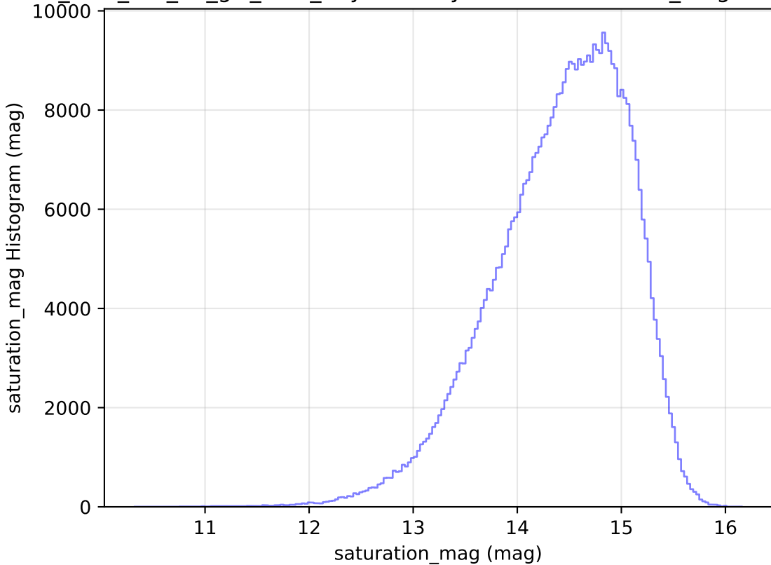
too_elab_r64_d3_giz_v3.4_10yrs All sky i band: saturation_mag Histogram
