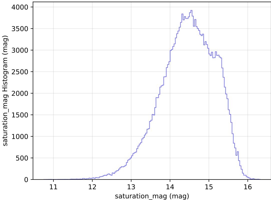
too_elab_r64_d3_giz_v3.4_10yrs All sky g band: saturation_mag Histogram
