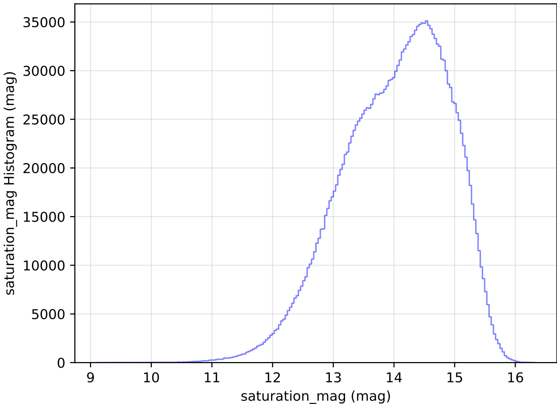
too_elab_r64_d3_giz_v3.4_10yrs All sky all bands: saturation_mag Histogram
