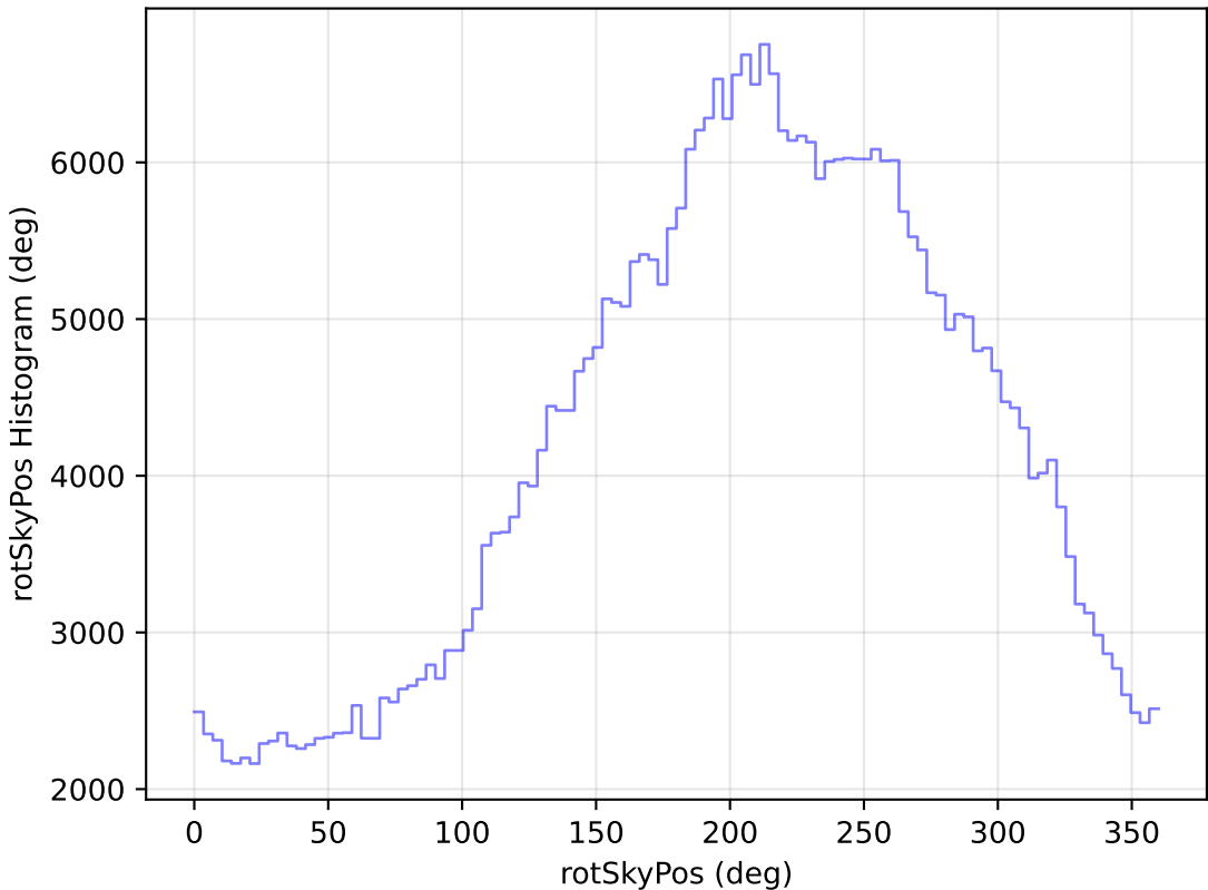
too_elab_r64_d3_giz_v3.4_10yrs WFD z band: rotSkyPos Histogram
