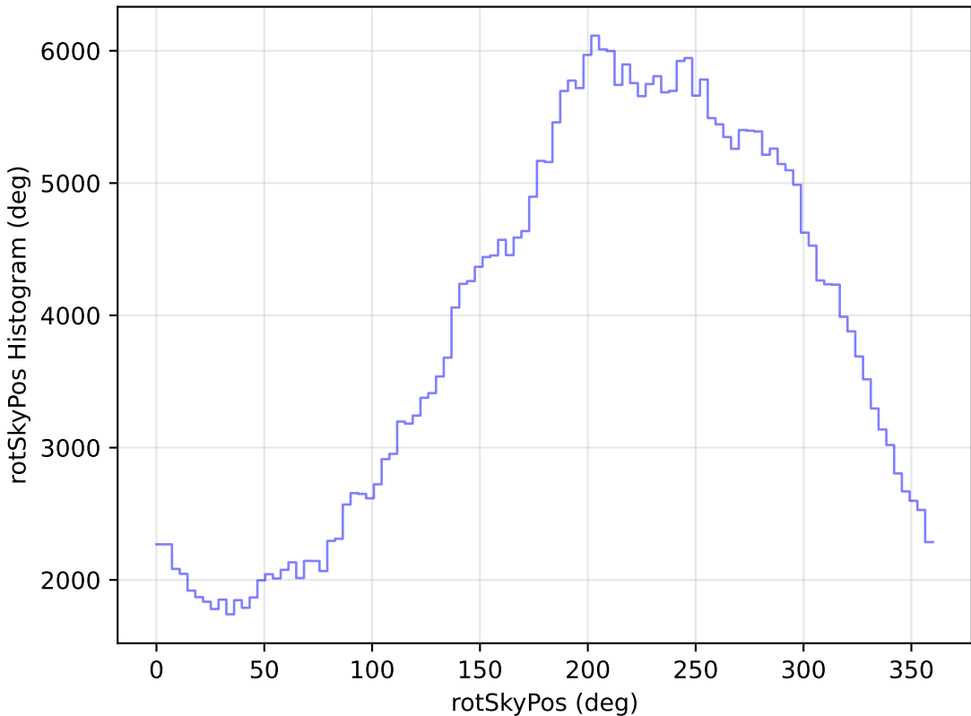
too_elab_r64_d3_giz_v3.4_10yrs WFD y band: rotSkyPos Histogram
