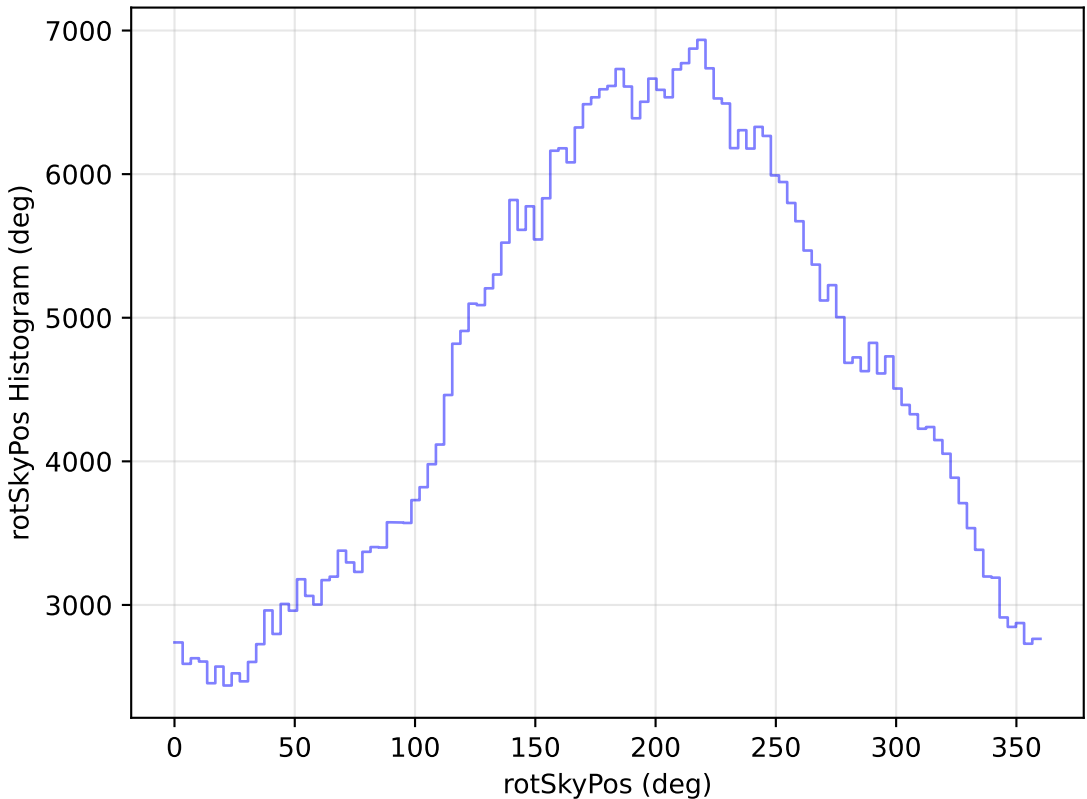
too_elab_r64_d3_giz_v3.4_10yrs WFD r band: rotSkyPos Histogram
