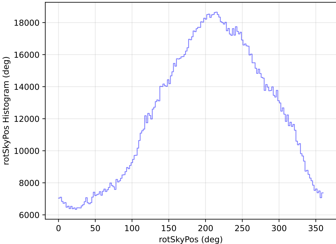
too_elab_r64_d3_giz_v3.4_10yrs WFD all bands: rotSkyPos Histogram
