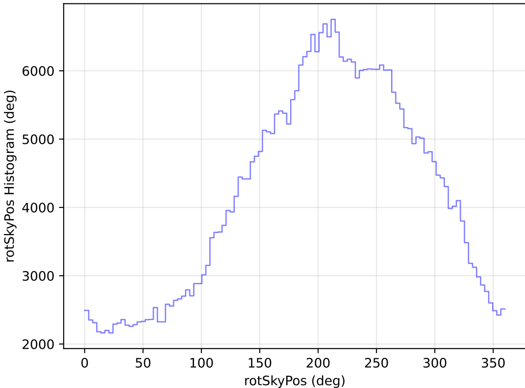
too_elab_r64_d3_giz_v3.4_10yrs All sky z band: rotSkyPos Histogram
