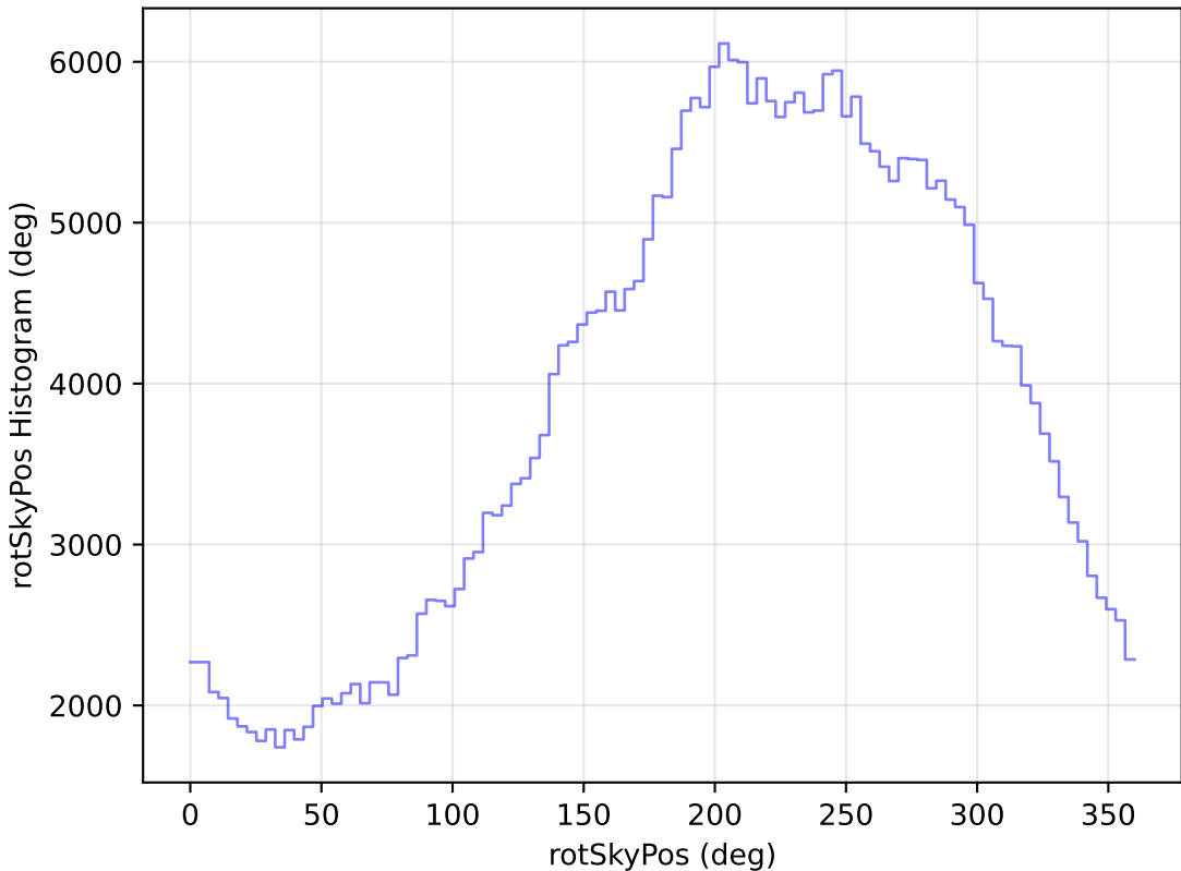
too_elab_r64_d3_giz_v3.4_10yrs All sky y band: rotSkyPos Histogram
