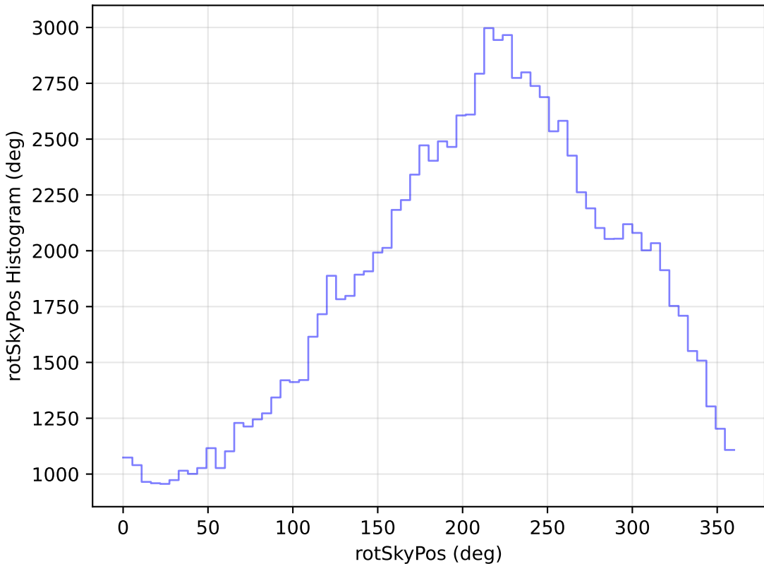
too_elab_r64_d3_giz_v3.4_10yrs All sky u band: rotSkyPos Histogram
