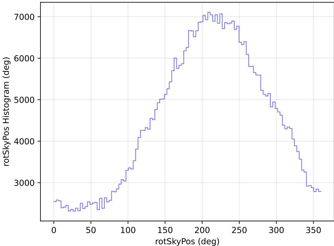
too_elab_r64_d3_giz_v3.4_10yrs All sky i band: rotSkyPos Histogram
