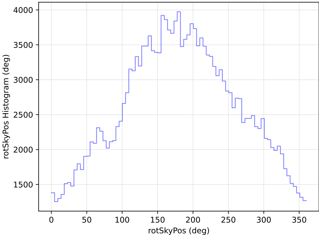
too_elab_r64_d3_giz_v3.4_10yrs All sky g band: rotSkyPos Histogram
