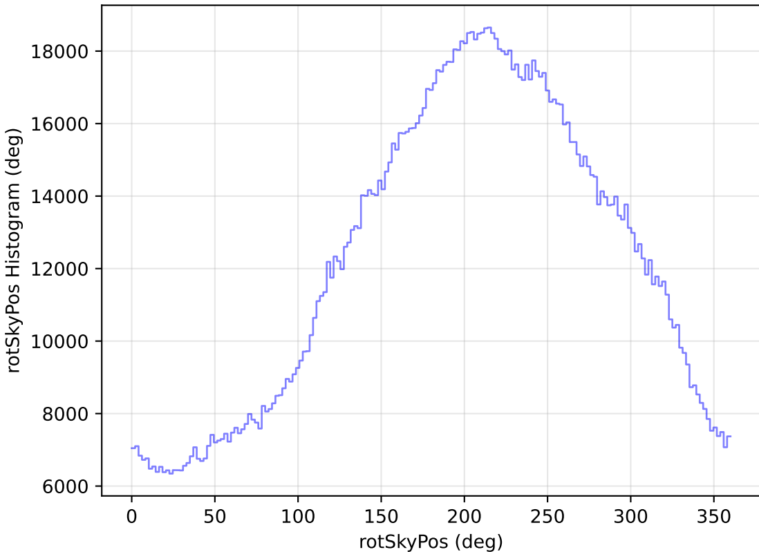
too_elab_r64_d3_giz_v3.4_10yrs All sky all bands: rotSkyPos Histogram
