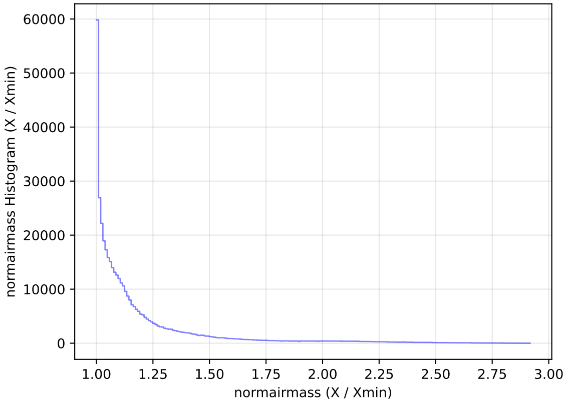
too_elab_r64_d3_giz_v3.4_10yrs WFD z band: normairmass Histogram
