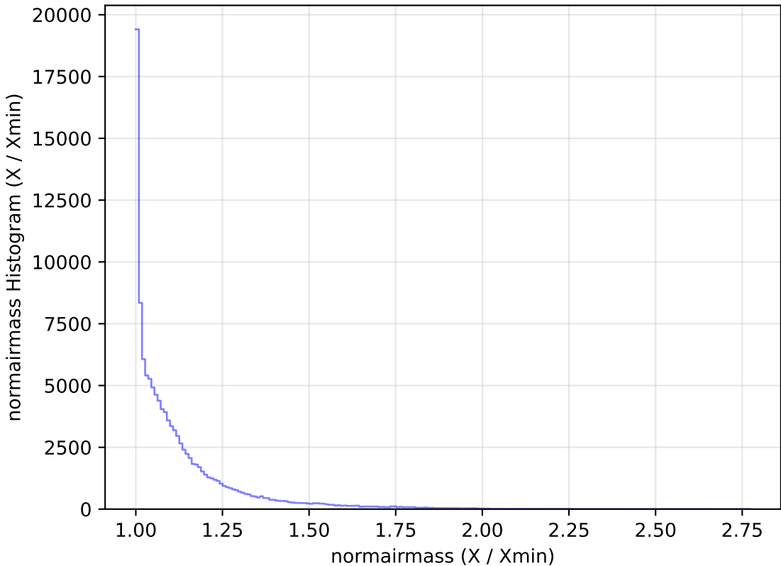
too_elab_r64_d3_giz_v3.4_10yrs WFD u band: normairmass Histogram
