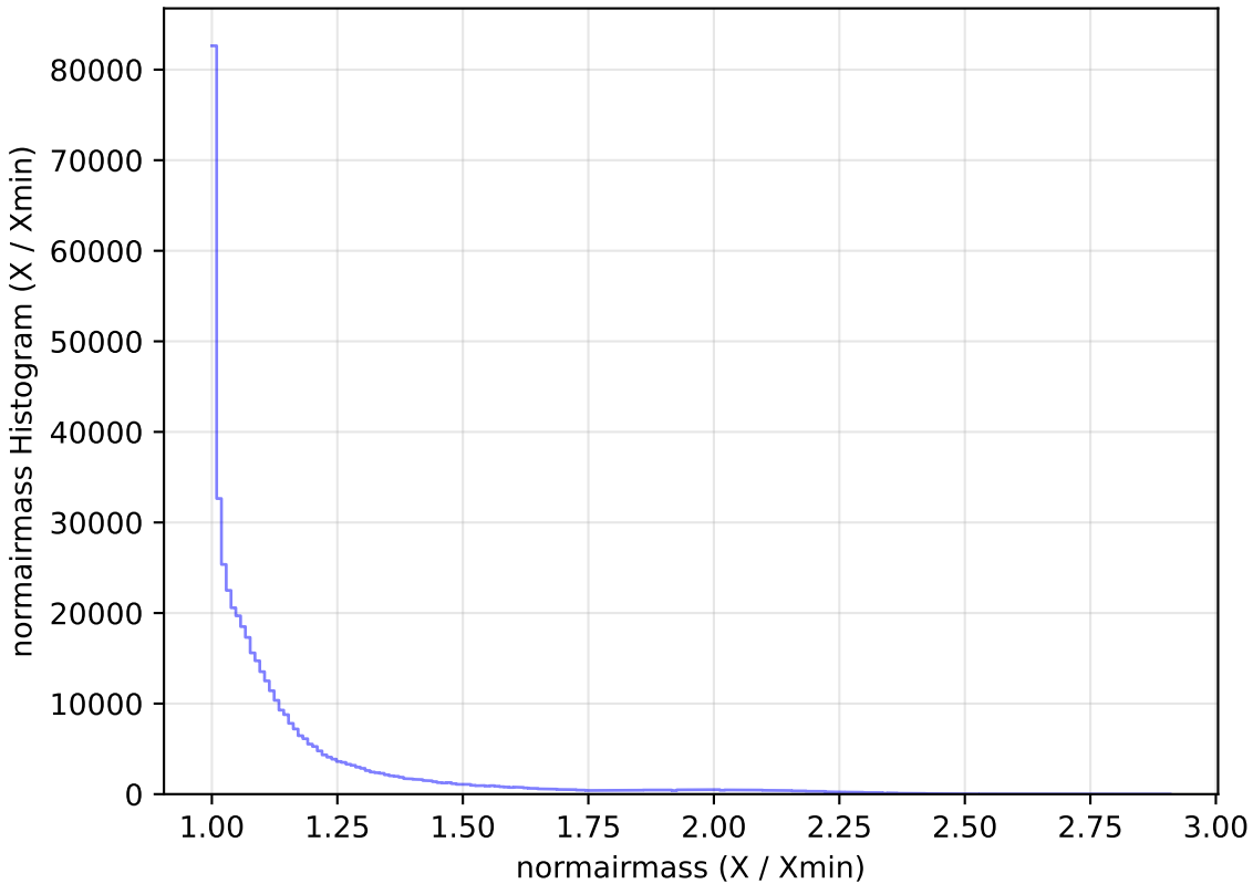
too_elab_r64_d3_giz_v3.4_10yrs WFD r band: normairmass Histogram
