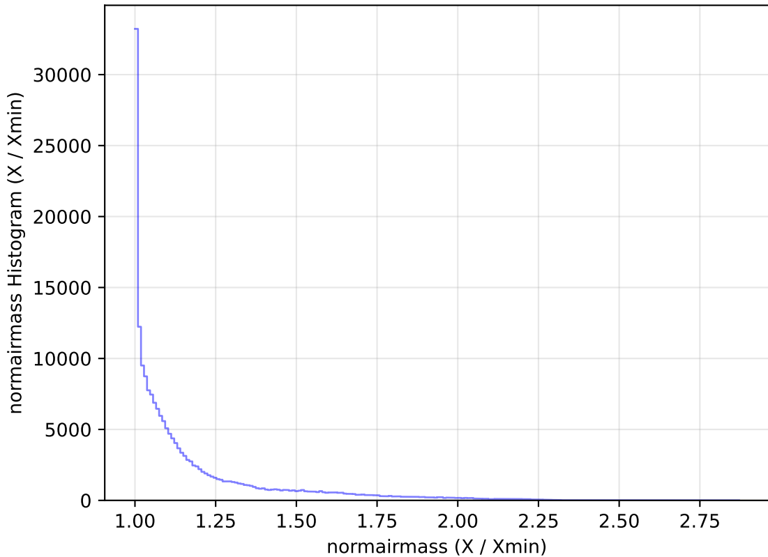
too_elab_r64_d3_giz_v3.4_10yrs WFD g band: normairmass Histogram
