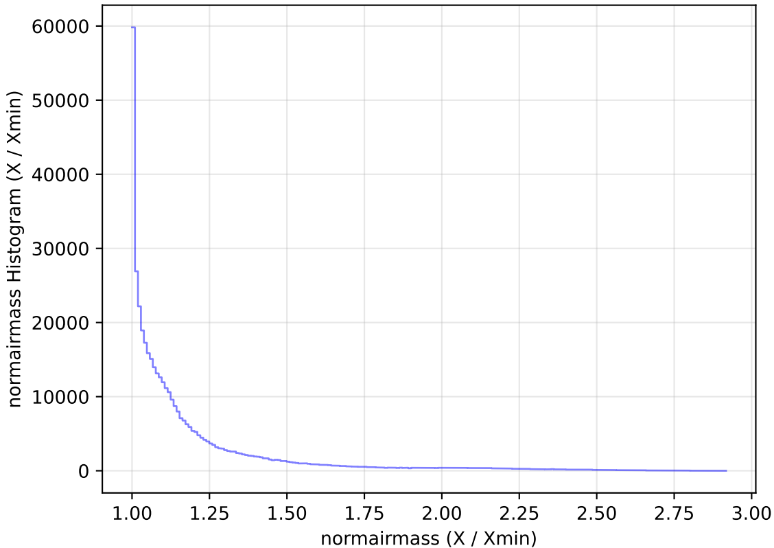
too_elab_r64_d3_giz_v3.4_10yrs All sky z band: normairmass Histogram
