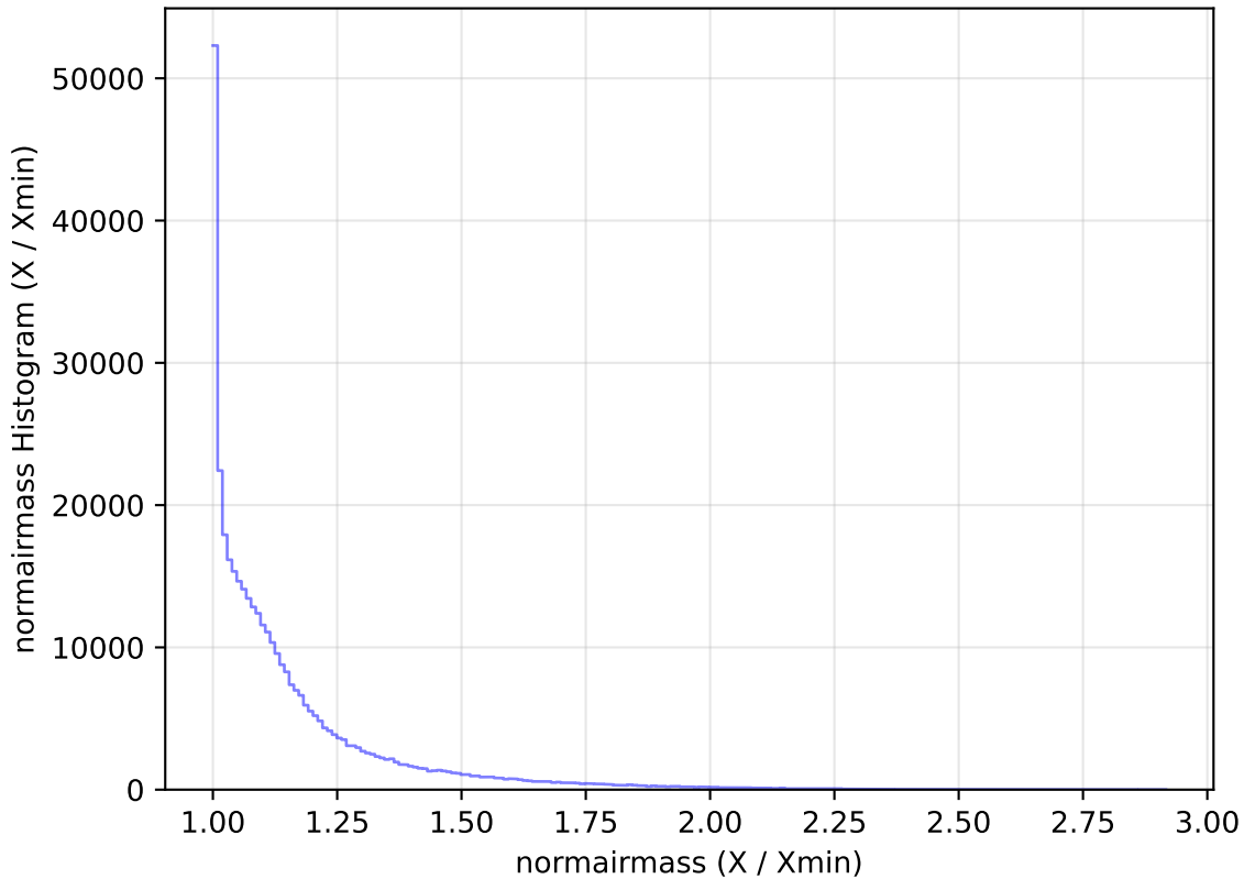
too_elab_r64_d3_giz_v3.4_10yrs All sky y band: normairmass Histogram
