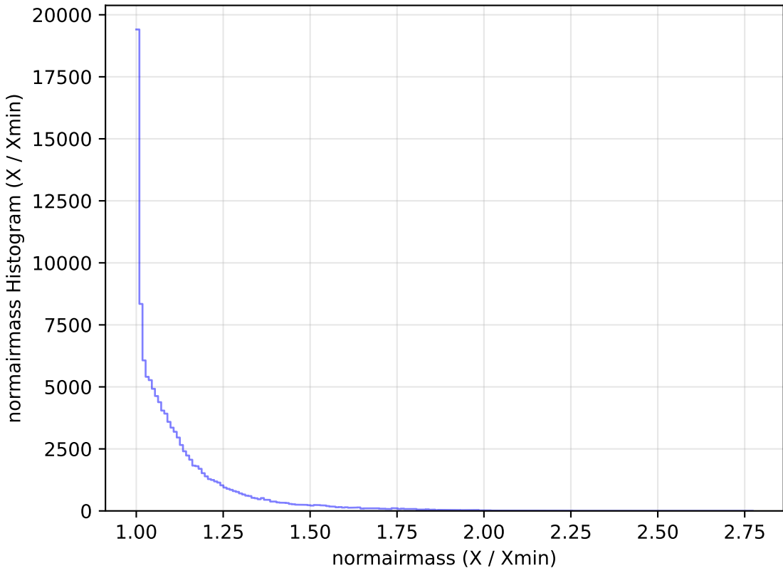
too_elab_r64_d3_giz_v3.4_10yrs All sky u band: normairmass Histogram
