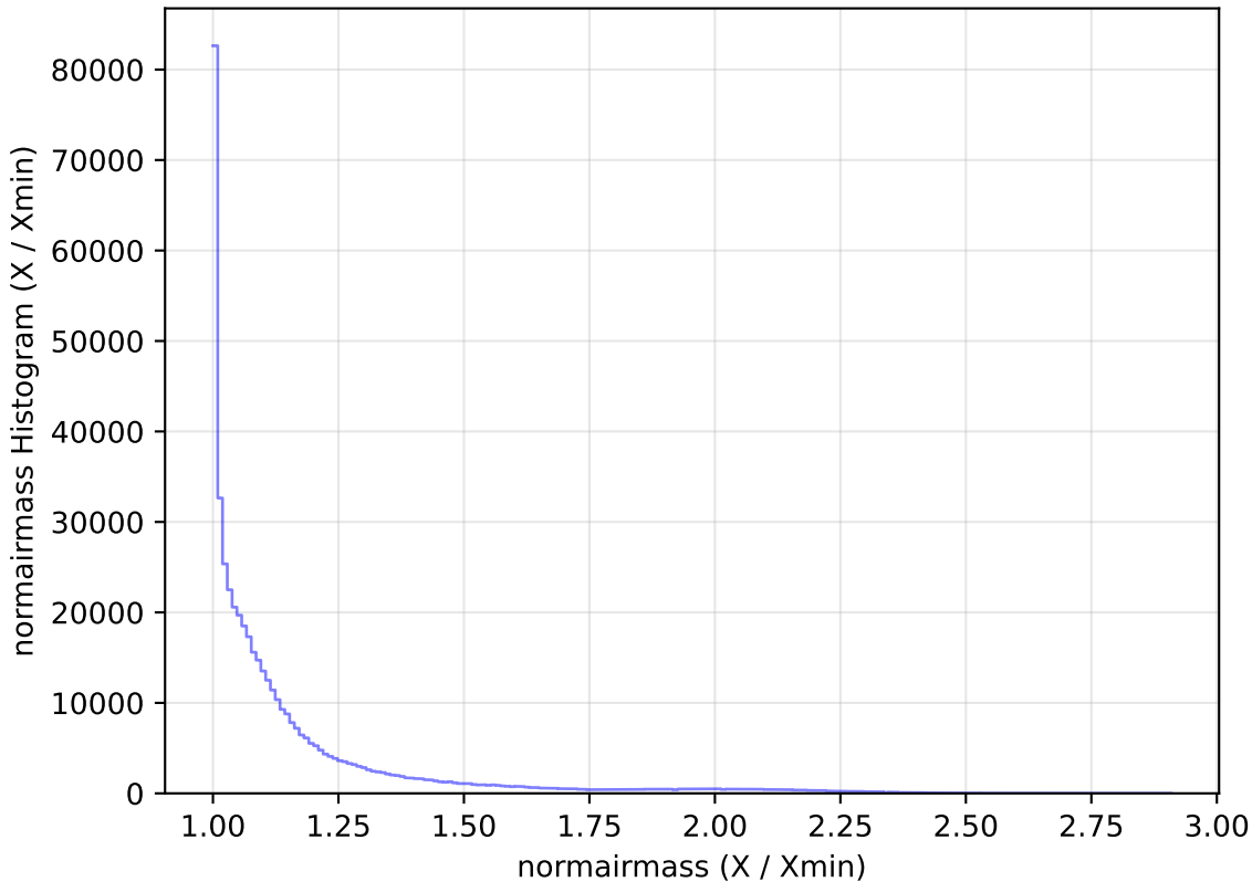
too_elab_r64_d3_giz_v3.4_10yrs All sky r band: normairmass Histogram
