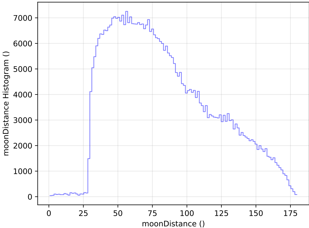
too_elab_r64_d3_giz_v3.4_10yrs WFD z band: moonDistance Histogram
