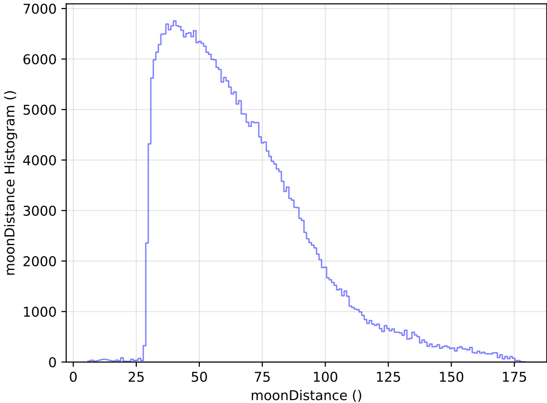
too_elab_r64_d3_giz_v3.4_10yrs WFD y band: moonDistance Histogram
