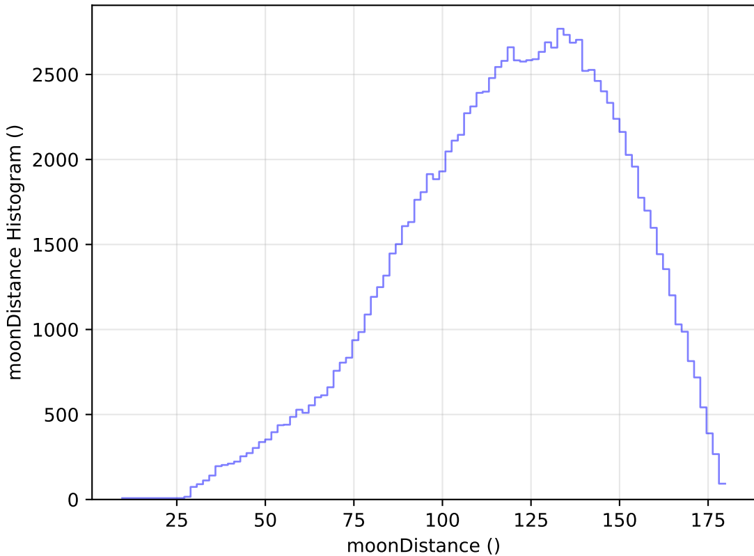
too_elab_r64_d3_giz_v3.4_10yrs WFD u band: moonDistance Histogram
