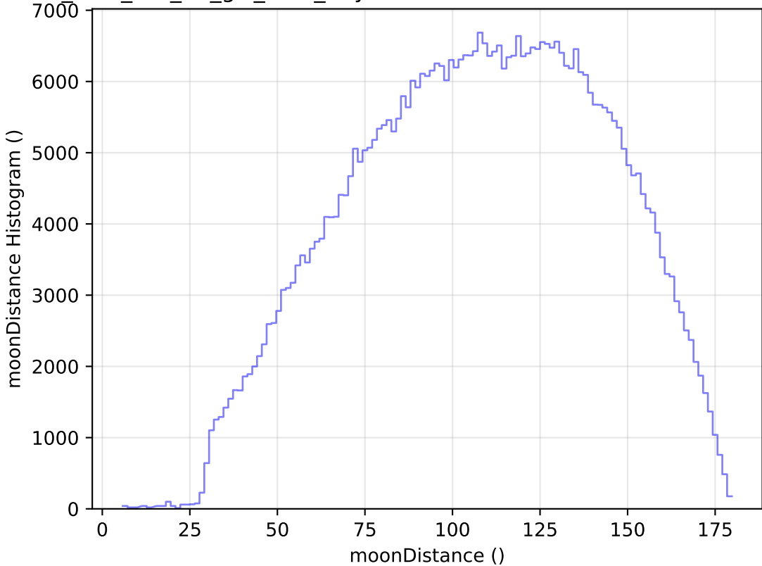
too_elab_r64_d3_giz_v3.4_10yrs WFD r band: moonDistance Histogram
