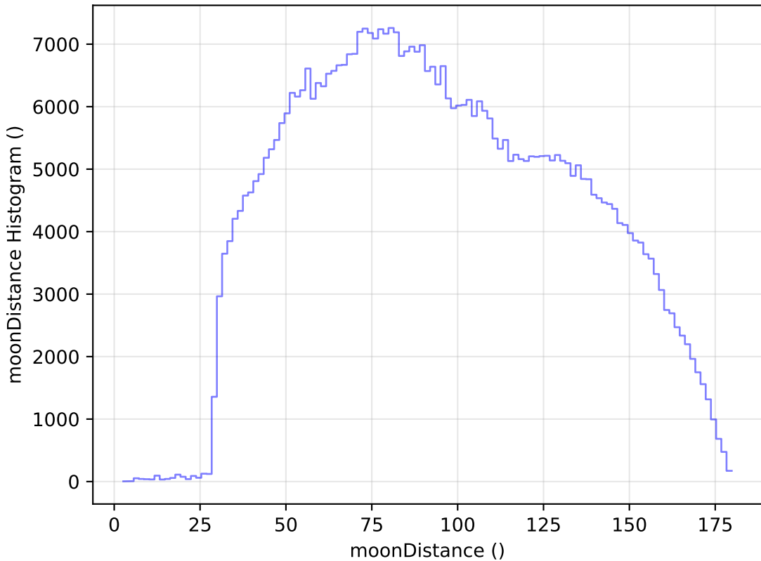
too_elab_r64_d3_giz_v3.4_10yrs WFD i band: moonDistance Histogram
