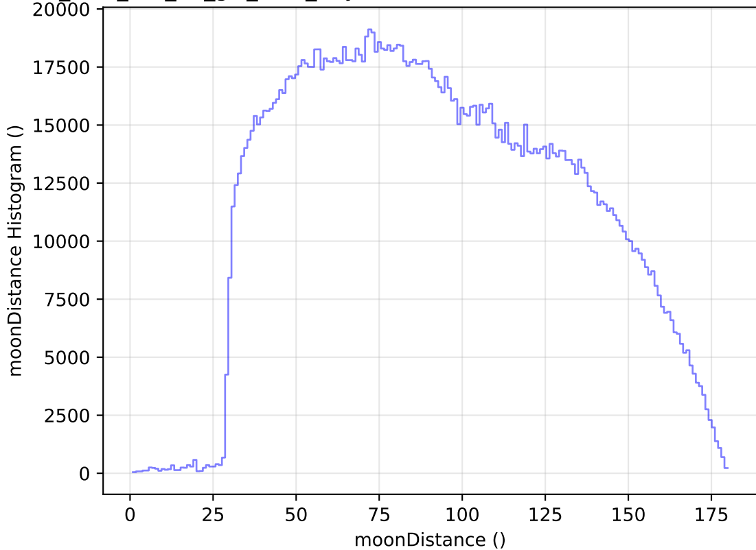
too_elab_r64_d3_giz_v3.4_10yrs WFD all bands: moonDistance Histogram
