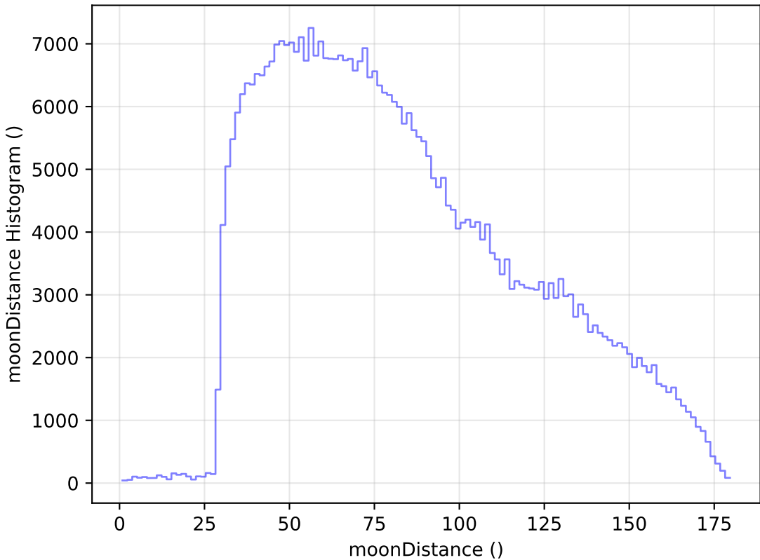
too_elab_r64_d3_giz_v3.4_10yrs All sky z band: moonDistance Histogram
