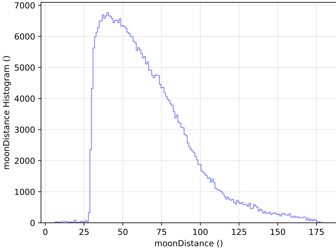
too_elab_r64_d3_giz_v3.4_10yrs All sky y band: moonDistance Histogram
