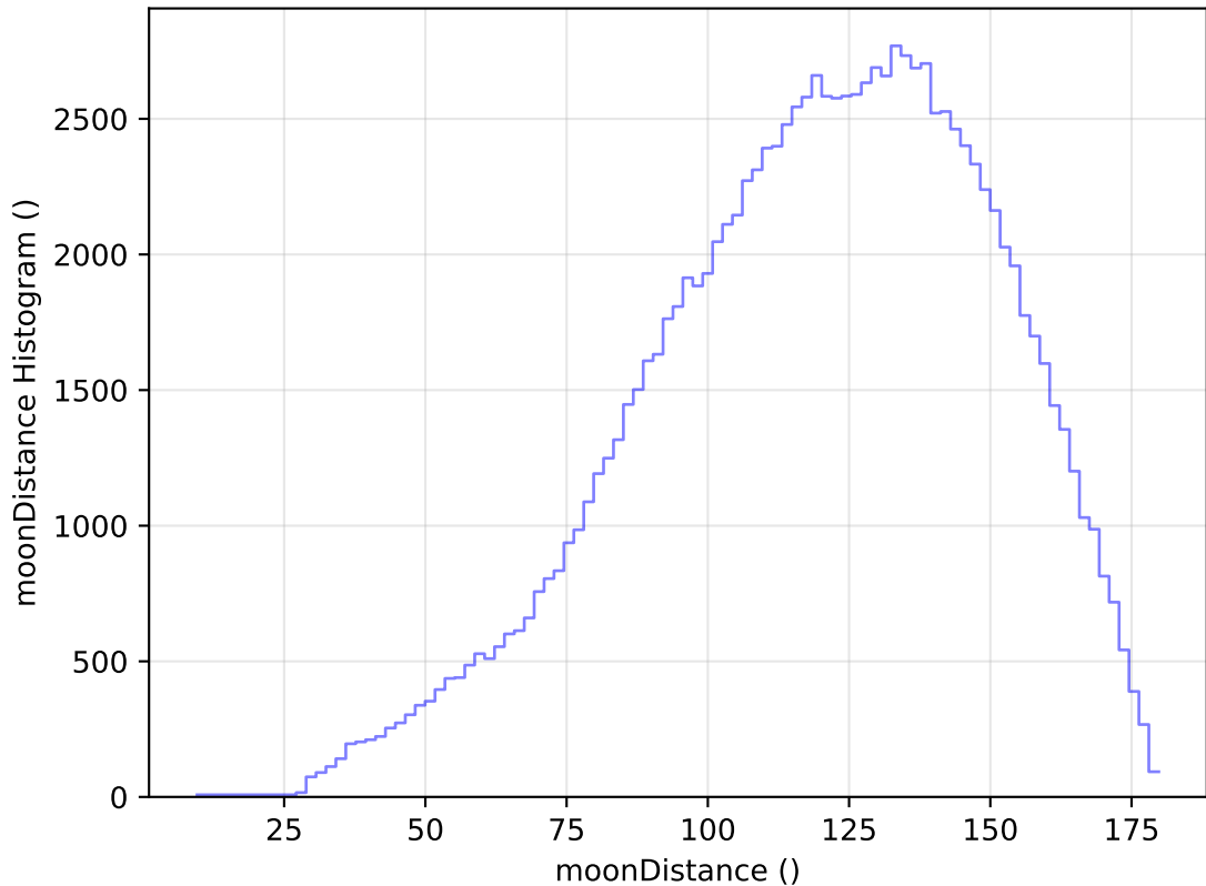
too_elab_r64_d3_giz_v3.4_10yrs All sky u band: moonDistance Histogram
