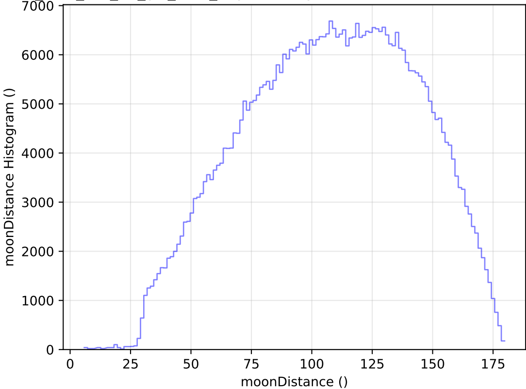
too_elab_r64_d3_giz_v3.4_10yrs All sky r band: moonDistance Histogram
