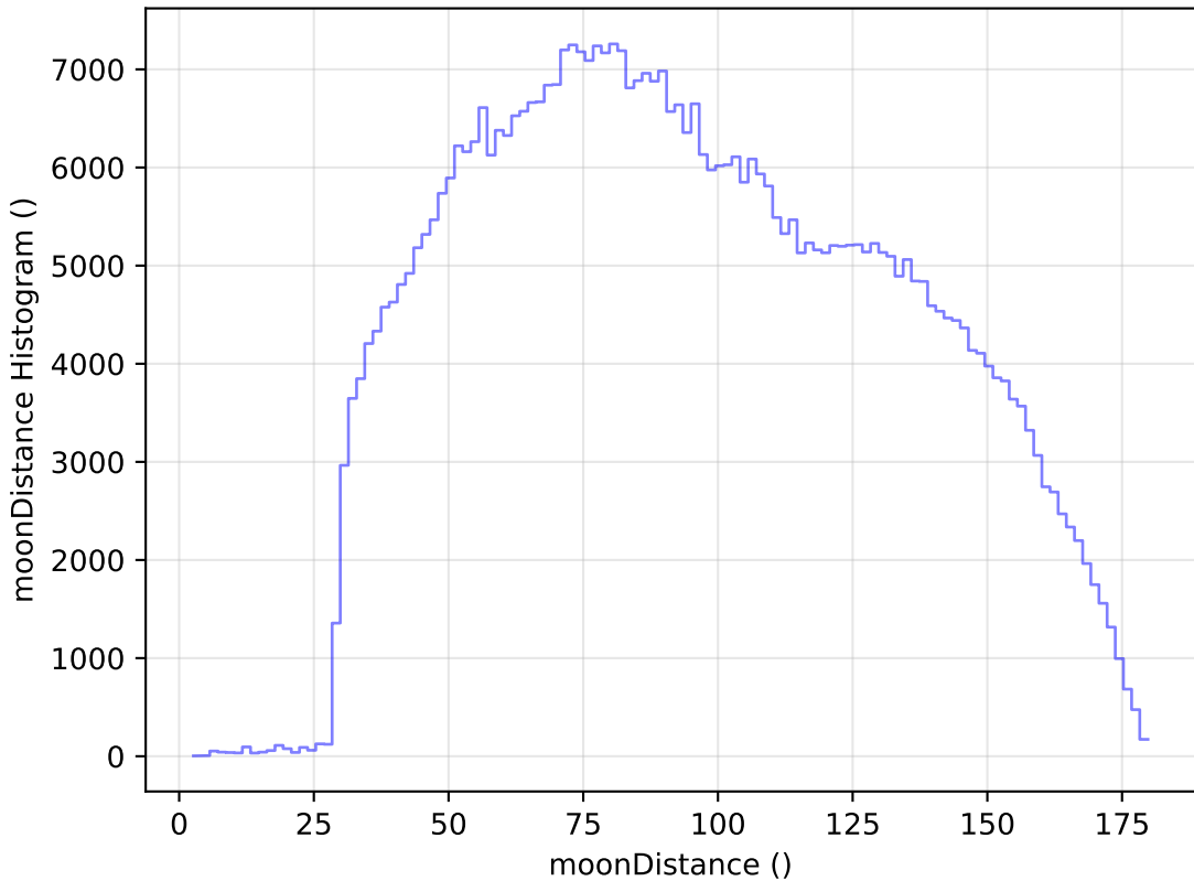
too_elab_r64_d3_giz_v3.4_10yrs All sky i band: moonDistance Histogram
