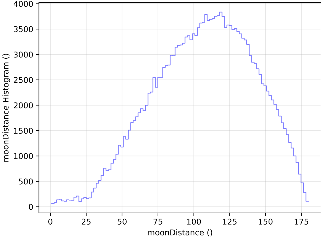
too_elab_r64_d3_giz_v3.4_10yrs All sky g band: moonDistance Histogram
