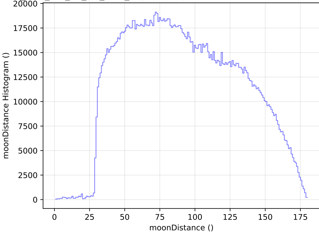
too_elab_r64_d3_giz_v3.4_10yrs All sky all bands: moonDistance Histogram
