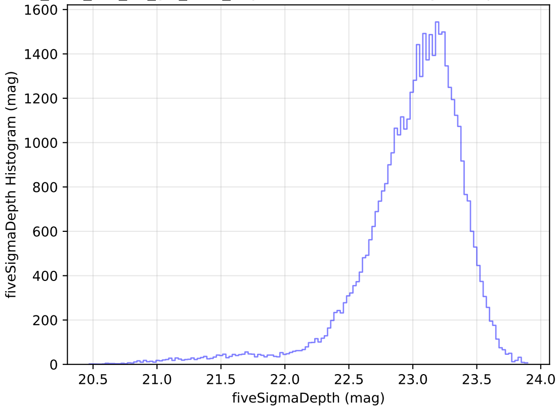
too_elab_r64_d3_giz_v3.4_10yrs Yr 1 z band: fiveSigmaDepth Histogram
