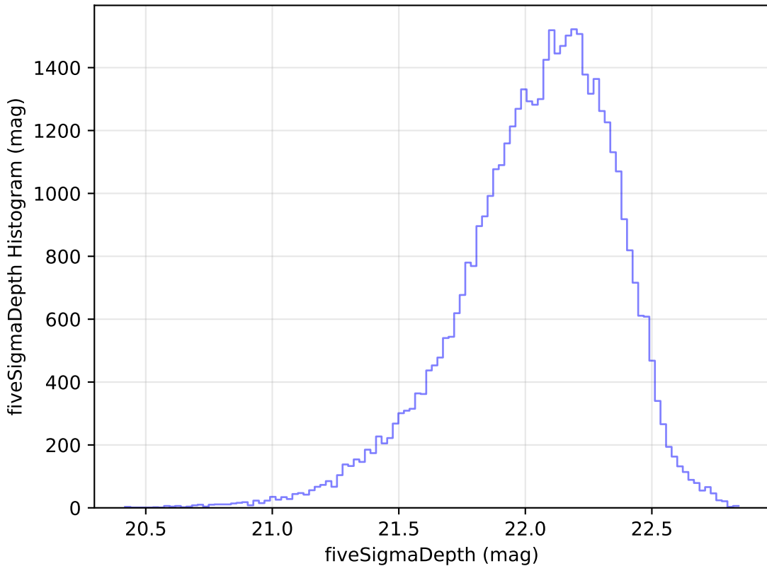
too_elab_r64_d3_giz_v3.4_10yrs Yr 1 y band: fiveSigmaDepth Histogram
