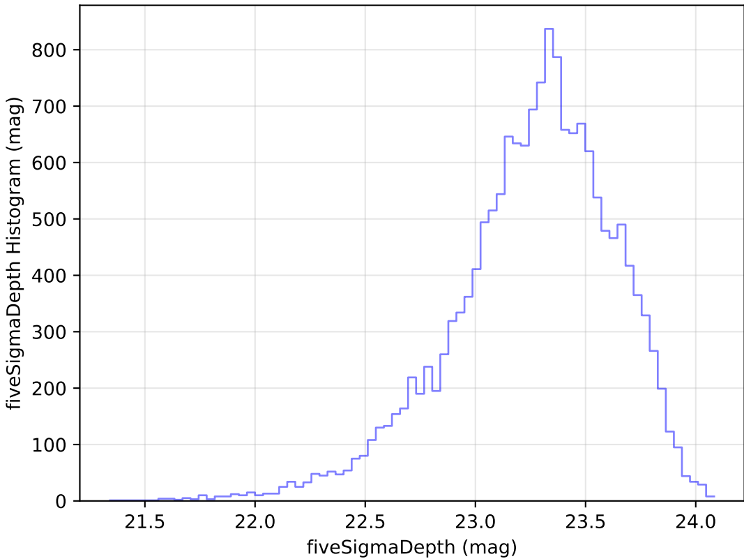
too_elab_r64_d3_giz_v3.4_10yrs Yr 1 u band: fiveSigmaDepth Histogram
