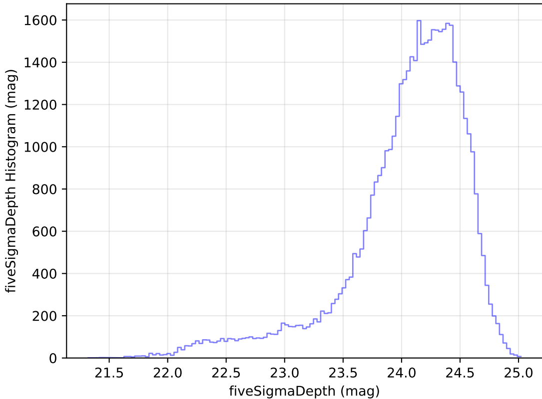
too_elab_r64_d3_giz_v3.4_10yrs Yr 1 r band: fiveSigmaDepth Histogram
