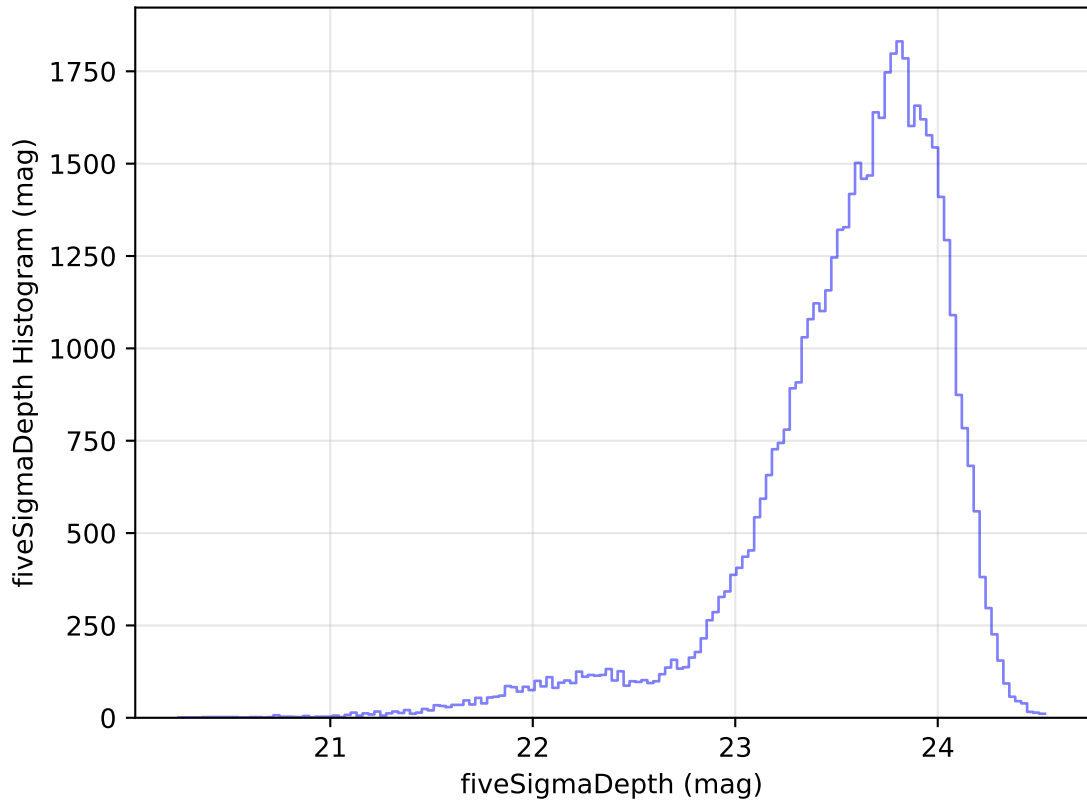
too_elab_r64_d3_giz_v3.4_10yrs Yr 1 i band: fiveSigmaDepth Histogram
