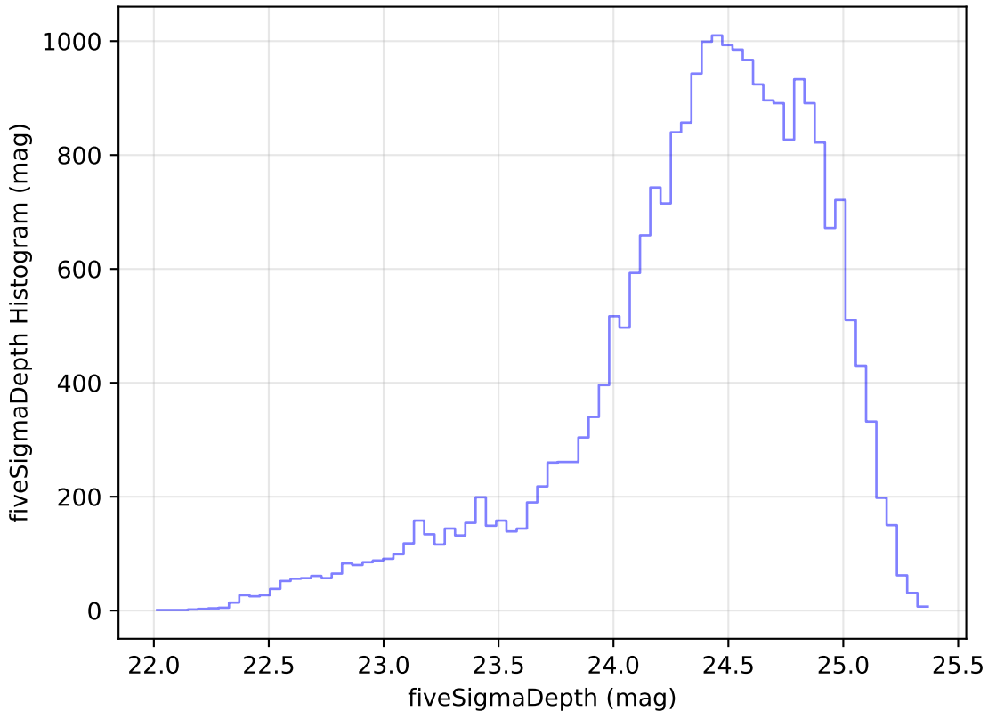
too_elab_r64_d3_giz_v3.4_10yrs Yr 1 g band: fiveSigmaDepth Histogram
