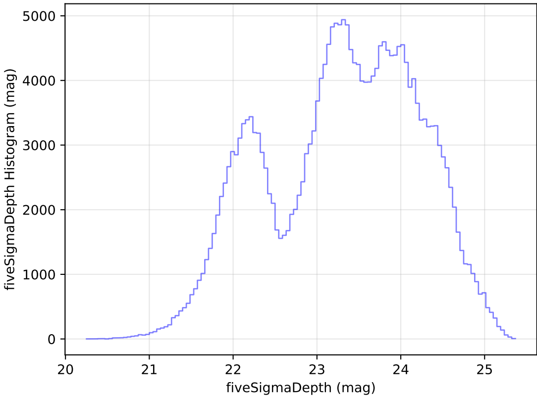
too_elab_r64_d3_giz_v3.4_10yrs Yr 1 all bands: fiveSigmaDepth Histogram
