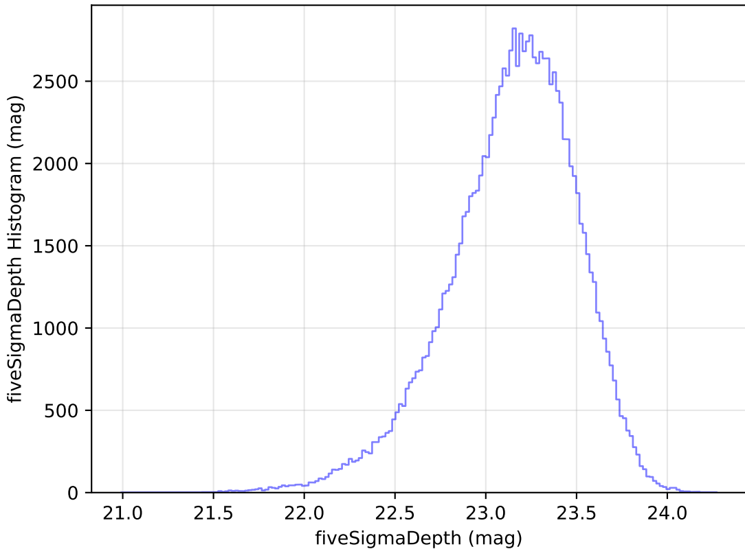
too_elab_r64_d3_giz_v3.4_10yrs WFD u band: fiveSigmaDepth Histogram
