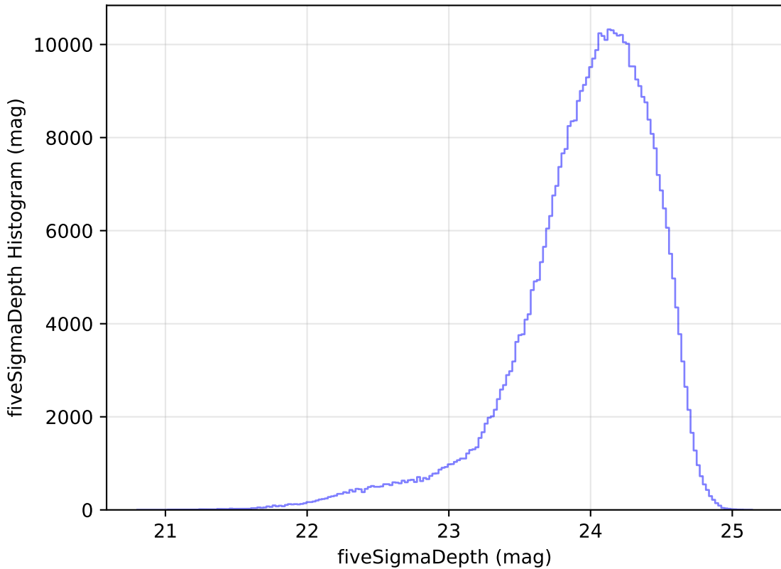
too_elab_r64_d3_giz_v3.4_10yrs WFD r band: fiveSigmaDepth Histogram
