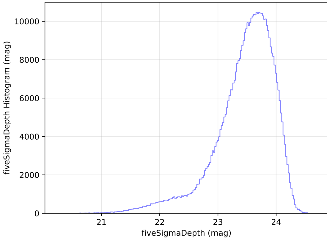
too_elab_r64_d3_giz_v3.4_10yrs WFD i band: fiveSigmaDepth Histogram
